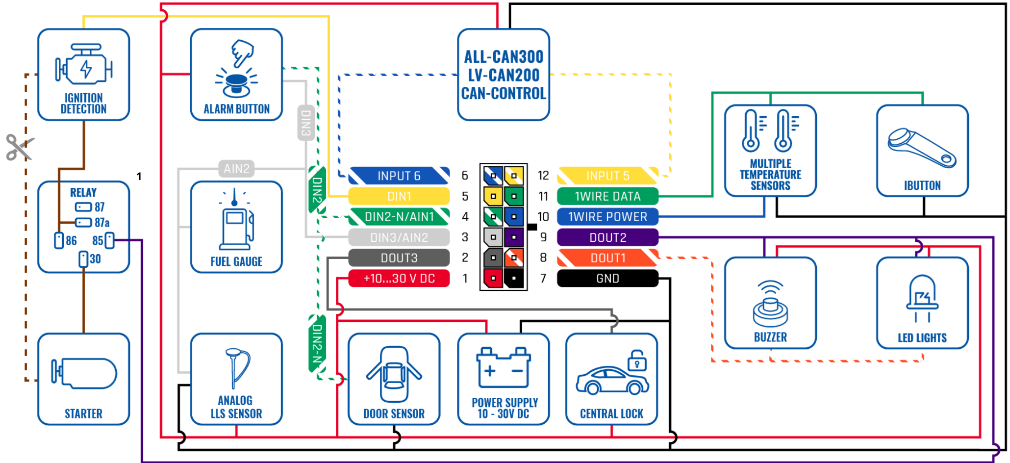
Figure 2 FMM230 Wiring scheme
