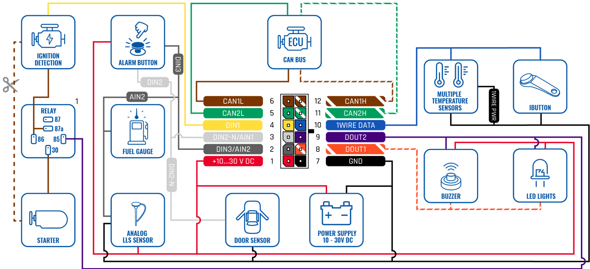
Figure 3 FMB240 Wiring scheme
