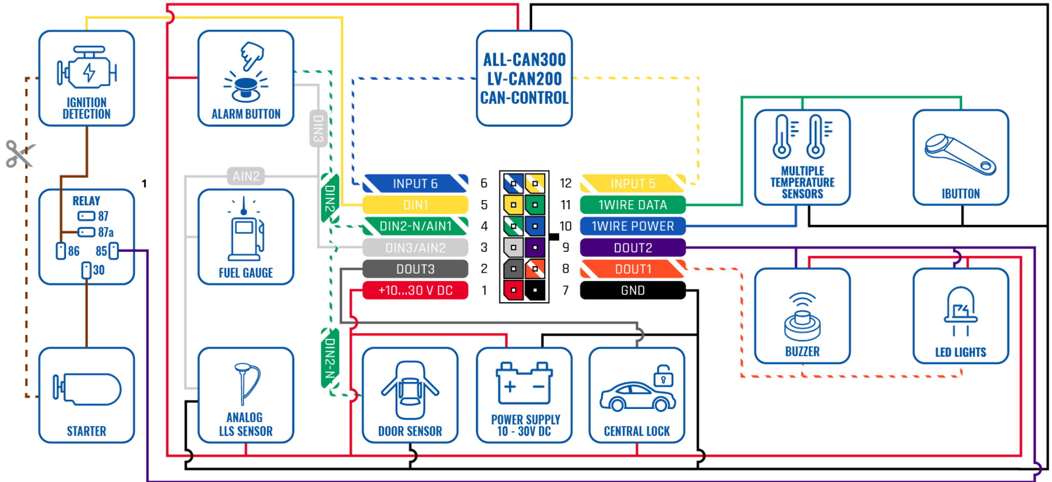
Figure 3 FMB230 Wiring scheme
