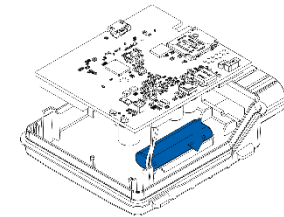
Figure 5 Cover removal
